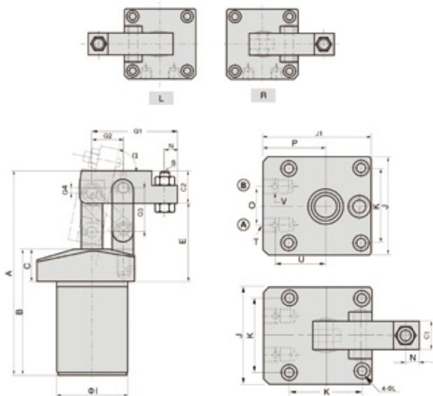
(A) CLAMPING PORT (B) UNCLAMPING PORT
