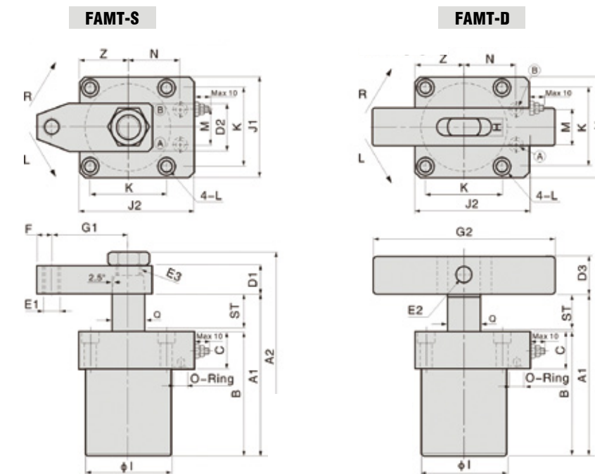
Ⓐ CLAMPING PORT Ⓑ UNCLAMPING PORT
