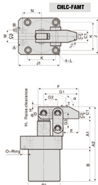
(A) CLAMPING PORT (B) UNCLAMPING PORT
