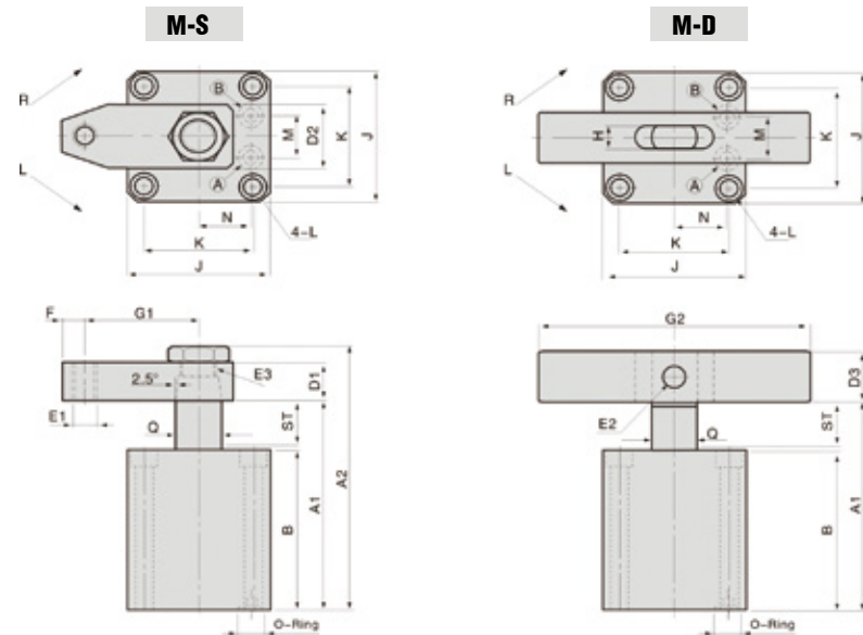
Ⓐ CLAMPING PORT Ⓑ UNCLAMPING PORT
