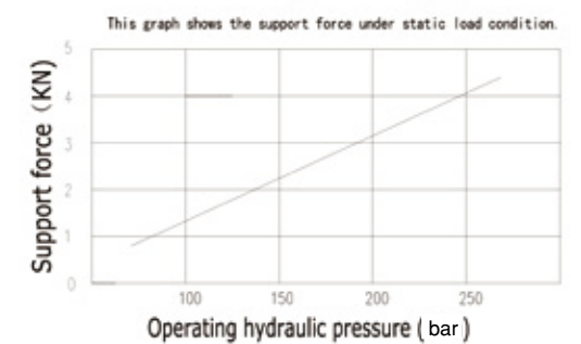
CSP-16 Support force graph
