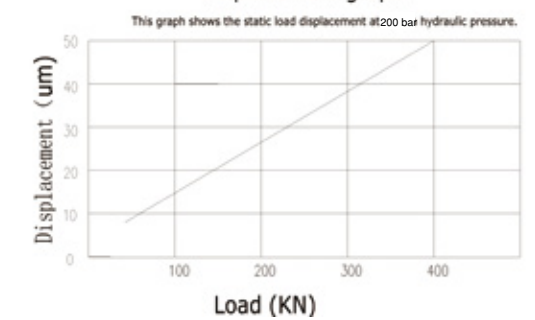
Displacement graph
