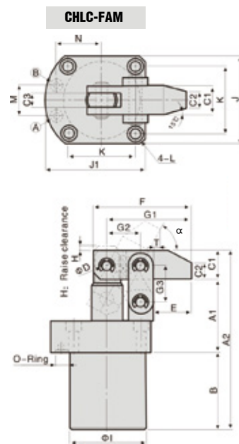
(A) CLAMPING PORT (B) UNCLAMPING PORT
