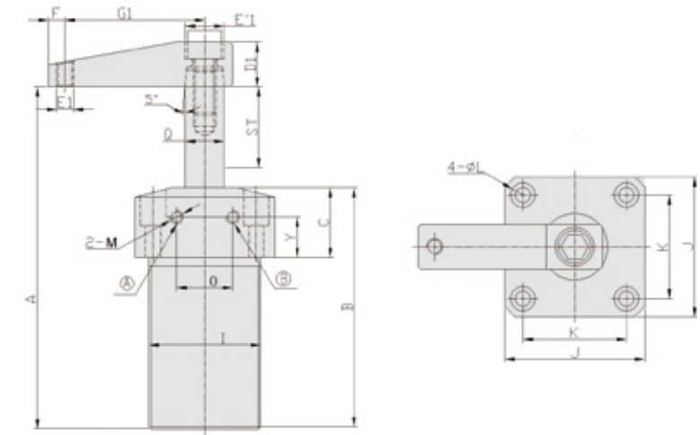
Ⓐ CLAMPING PORT Ⓑ UNCLAMPING PORT
