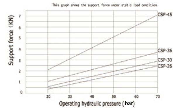
CSP-Support force graph
